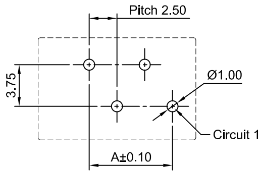
Even Numbers Component Side [A7921WVI-XP-**-2]
