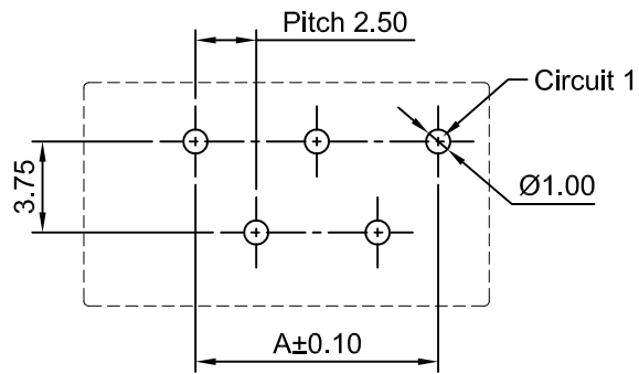
Odd Numbers Component Side [A7921WVI-XP-**-2]
